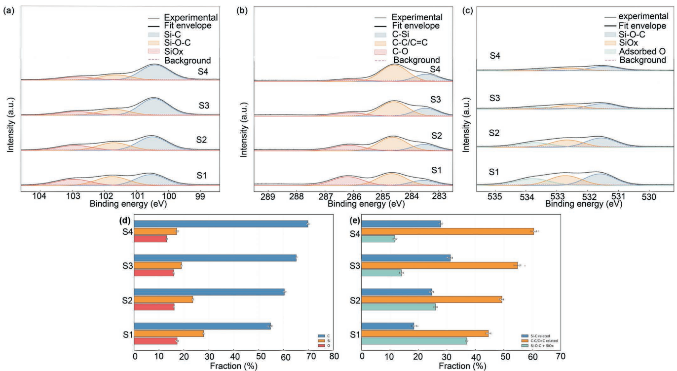
Fig. 3: XPS evidence for chemical-state regulation in the amorphous silicon-carbon nanocomposite sensing layers. (a) High-resolution Si 2p spectra with fitted Si-C and oxygen-containing silicon components. (b) High-resolution C 1s spectra distinguishing C-C/C=C and carbon bonded to silicon or oxygen. (c) High-resolution O 1s spectra showing the decline of oxygen-rich bonding environments across the series. (d) Quantitative comparison of elemental atomic fractions of C, Si, and O. (e) Quantitative comparison of Si-C related, C-C/C=C related, and Si-O-C plus SiOx bond-state fractions.
