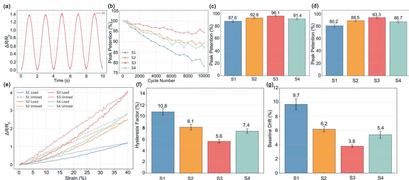
Fig. 9: Long-term durability and hysteresis characteristics of the flexible strain sensors. (a) Representative cyclic waveform window during repeated loading. (b) Peak-retention curves as a function of cycle number. (c) Peak retention at 5000 cycles. (d) Peak retention at 10000 cycles. (e) Loading-unloading hysteresis loops at 40% strain. (f) Hysteresis-factor comparison. (g) Baseline drift after long-cycle testing.
