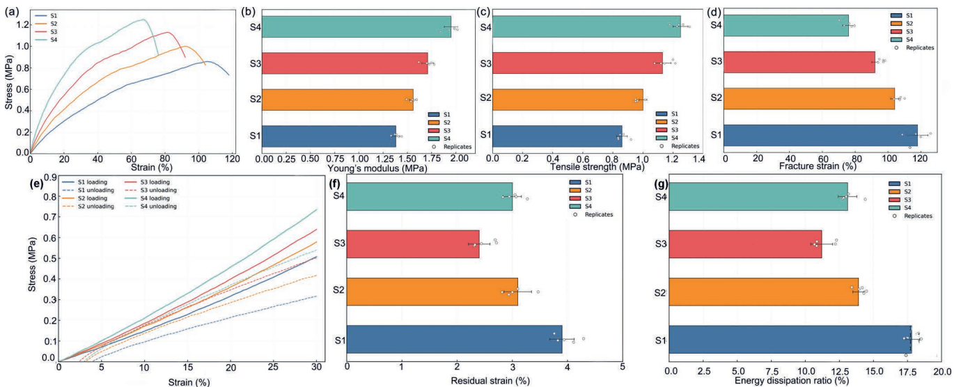
Fig. 6: Mechanical behavior and cyclic mechanical reversibility of the nanocomposite sensing layers. (a) Stress-strain curves of S1 – S4. (b) Comparison of Young's modulus. (c) Comparison of tensile strength. (d) Comparison of fracture strain. (e) Representative cyclic loading-unloading response at 30 % strain. (f) Residual strain after 100 cycles. (g) Mechanical energy dissipation ratio. Together, these panels show that S3 combines sufficient flexibility with the best mechanical reversibility in the operating range.
