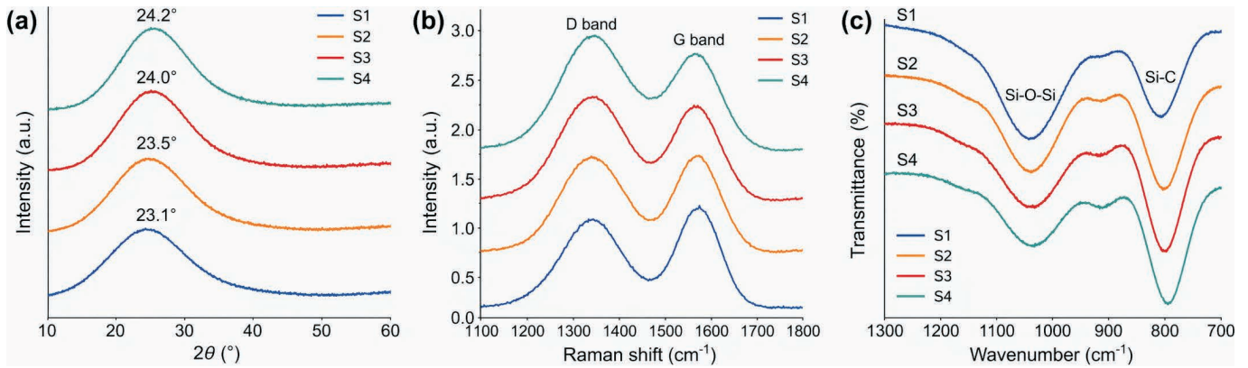
Fig. 2: Structural evolution of the amorphous silicon-carbon network revealed by means of XRD, Raman spectroscopy, and FTIR. (a) XRD patterns of S1 – S4 showing broad amorphous halos without sharp crystalline peaks. (b) Raman spectra with D and G bands marked for the four sensing layers. (c) FTIR spectra highlighting Si-C and Si-O-Si related vibrational regions.
