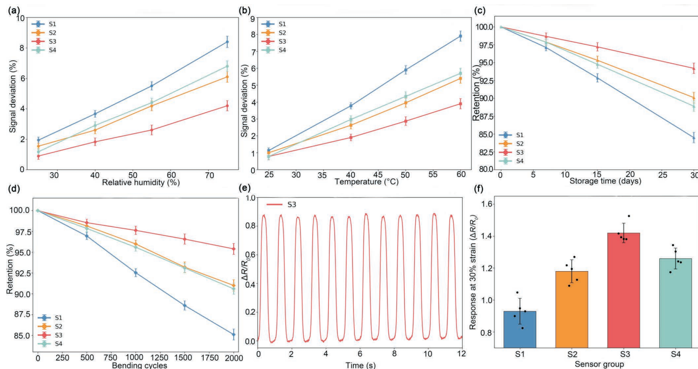
Fig. 10: Environmental robustness, bending endurance, and reproducibility of the nanocomposite strain sensors. (a) Humidity-dependent signal deviation. (b) Temperature-dependent signal deviation. (c) Storage retention after 30 days. (d) Retention after repeated bending. (e) Representative bending-cycle trace of the optimized sensor. (f) Batch-to-batch variation of device response.
