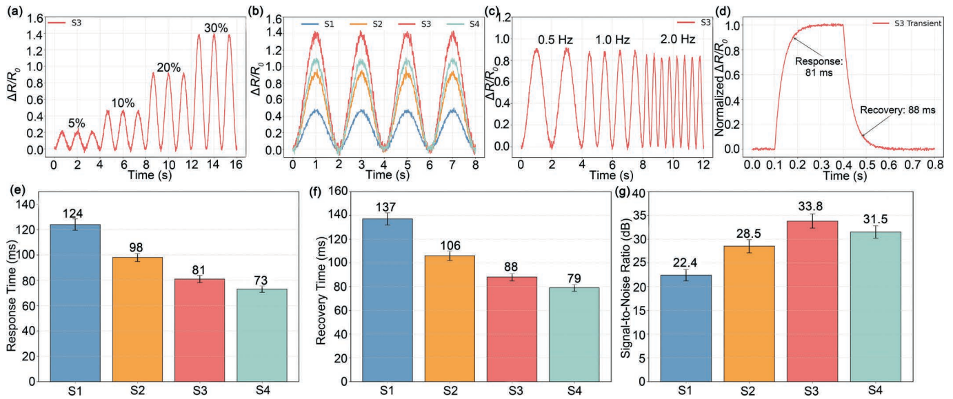
Fig. 8: Dynamic sensing behavior under variable strain amplitudes and loading frequencies. (a) Time-domain response of S3 at multiple strain amplitudes. (b) Comparative dynamic response of S1 – S4 at a fixed strain amplitude. (c) Frequency-dependent response of S3. (d) Enlarged transient response-recovery cycle of S3. (e) Response time comparison. (f) Recovery time comparison. (g) Signal-to-noise ratio at 5% strain.
