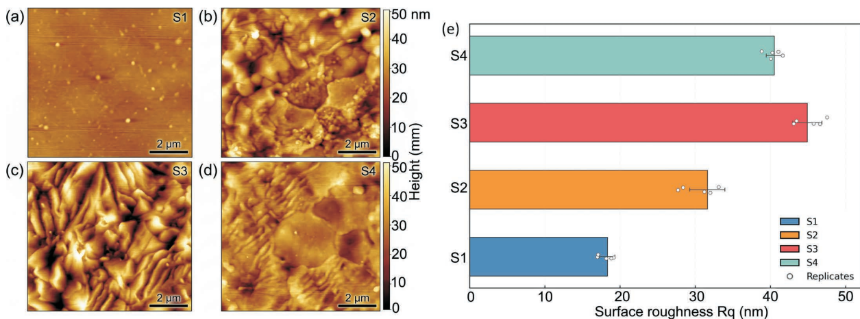
Fig. 5: AFM topography and roughness evolution of the sensing surfaces. (a – d) AFM height maps of S1, S2, S3, and S4. (e) Quantitative comparison of root-mean-square roughness R_q across S1 – S4. These panels demonstrate that moderate surface roughness and topographic heterogeneity are maximized in S3 and contribute to enhanced strain sensitivity.
