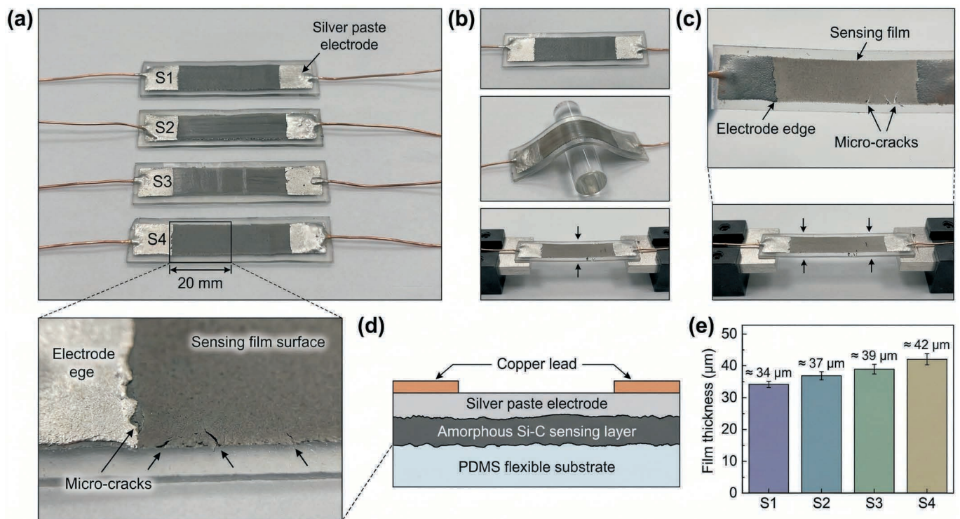
Fig. 1: Macroscopic appearance and geometric configuration of the flexible strain-sensor devices. (a) Photographs of the fabricated S1 – S4 devices under identical viewing conditions. (b) Flexibility demonstration of the representative device in flat, bent, and stretched states. (c) Enlarged view of the sensing region and electrode-transition region. (d) Cross-sectional device architecture showing the substrate, sensing layer, and electrode layout. (e) Quantitative comparison of film thickness across S1 – S4.
