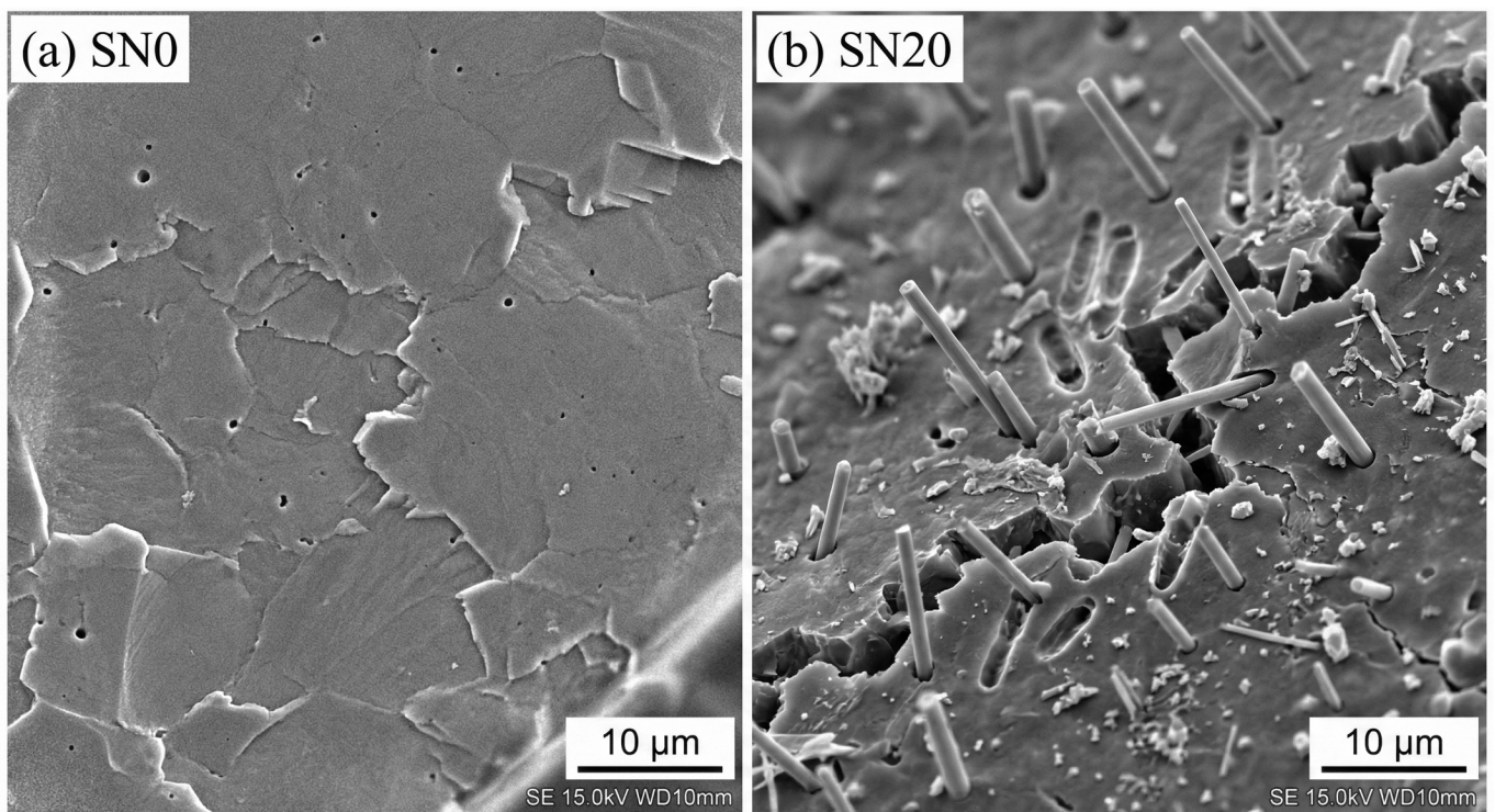
Fig. 3: Fracture surface morphology of (a) SN0 showing transgranular fracture and (b) SN20 exhibiting extensive whisker pull-out and crack deflection.
