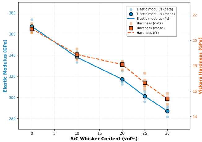
Fig. 7: Elastic modulus and hardness dependence on SiC whisker volume fraction.
