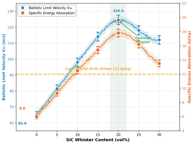
Fig. 9: Ballistic performance comparison of \text{Si}_3\text{N}_4 -SiC composites with varying whisker content.
