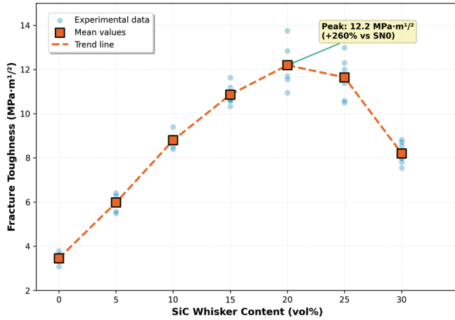
Fig. 6: Fracture toughness variation with whisker content, demonstrating 260 % improvement at optimal composition.
