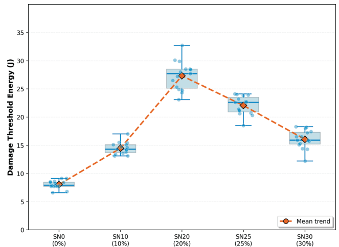
Fig. 8: Drop-weight impact test results showing damage threshold energy for different compositions.
