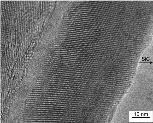
Fig. 4: High-resolution TEM image of \text{Si}_3\text{N}_4 -SiC interface showing amorphous intergranular film and crystallographic orientation relationship.
