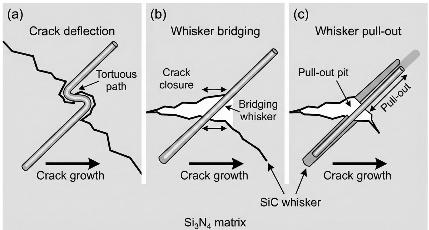
Fig. 10: Schematic illustration of toughening mechanisms: (a) crack deflection, (b) whisker bridging, and (c) whisker pull-out.
