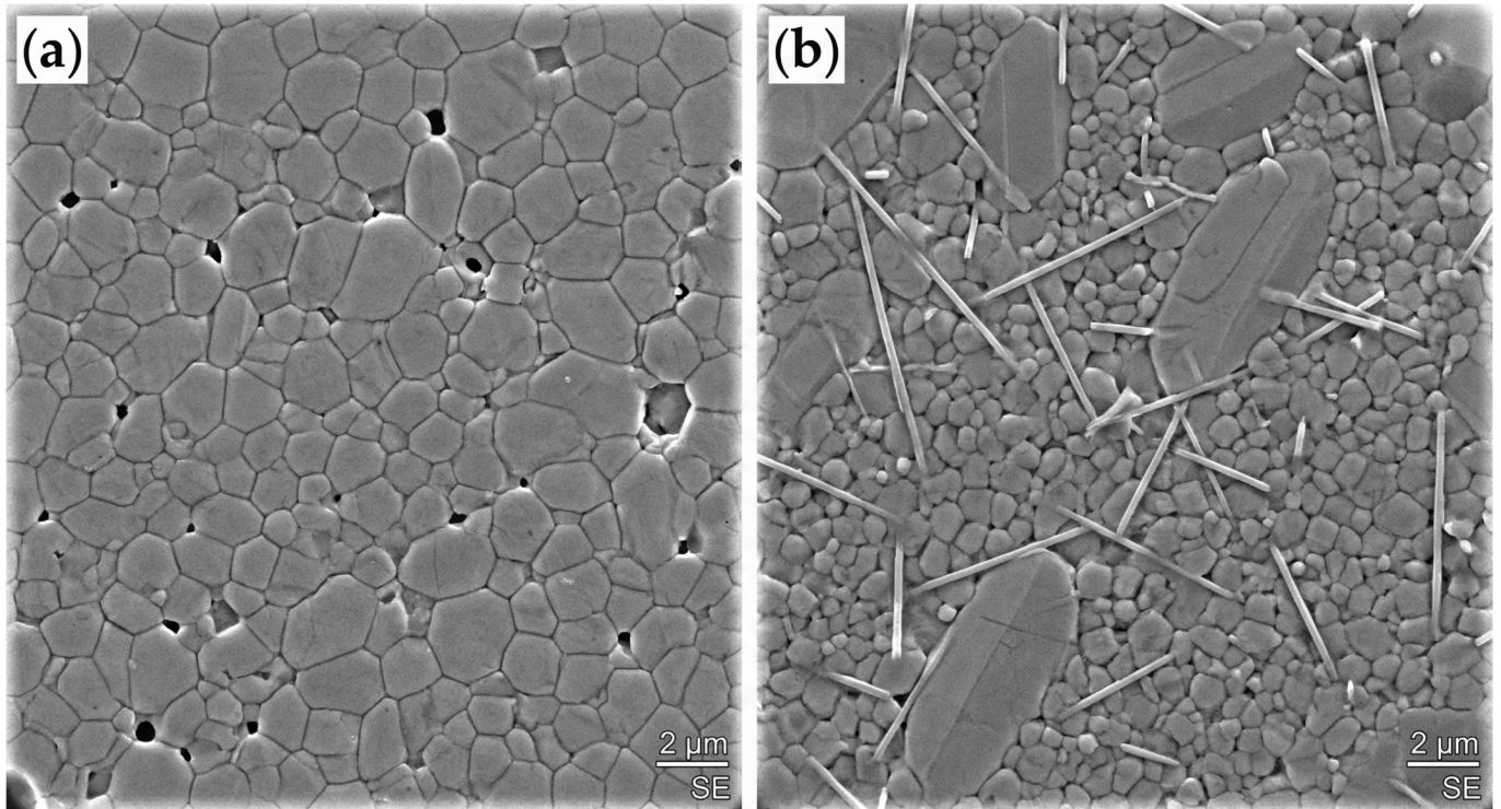
Fig. 2: SEM micrographs of (a) monolithic \text{Si}_3\text{N}_4 (SN0) showing equiaxed grain structure and (b) SN20 composite with bimodal grain distribution and dispersed SiC whiskers.
