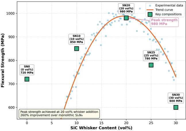
Fig. 5: Flexural strength as a function of SiC whisker content, showing peak strength at 20 vol% whisker addition.
