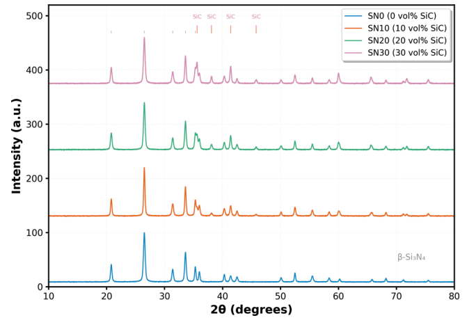
Fig. 1: X-ray diffraction patterns of Si 3 N 4 -SiC whisker composites showing β-Si 3 N 4 peaks and SiC reflections in whisker-containing samples.
